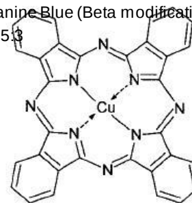
Structure III: Pigment Blue 15
